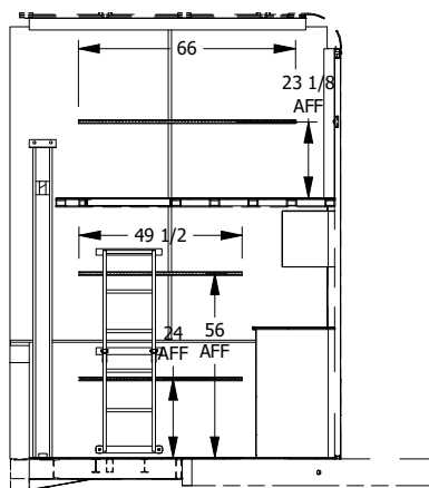
SECTION B-B SCALE 1/65
